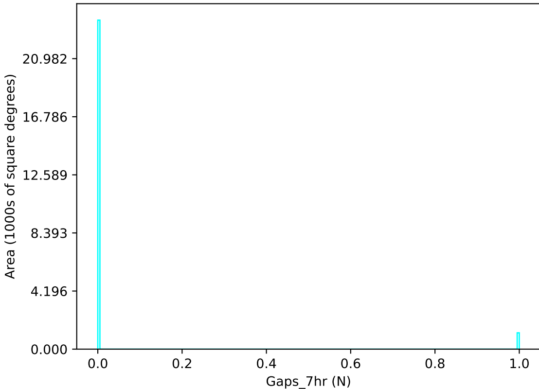
noroll_mjdp180_v3.4_10yrs u band: Gaps_7hr
