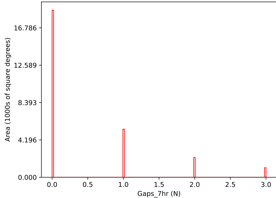
noroll_mjdp180_v3.4_10yrs i band: Gaps_7hr
