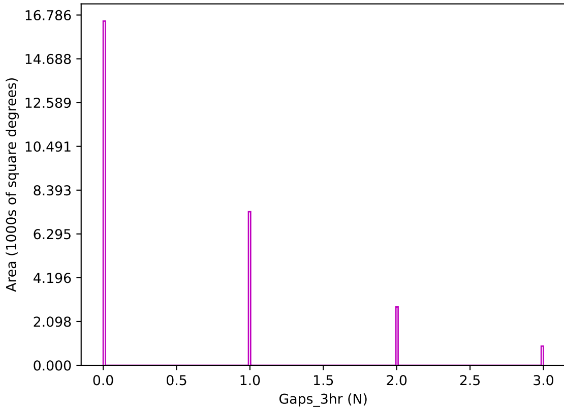
noroll_mjdp180_v3.4_10yrs z band: Gaps_3hr
