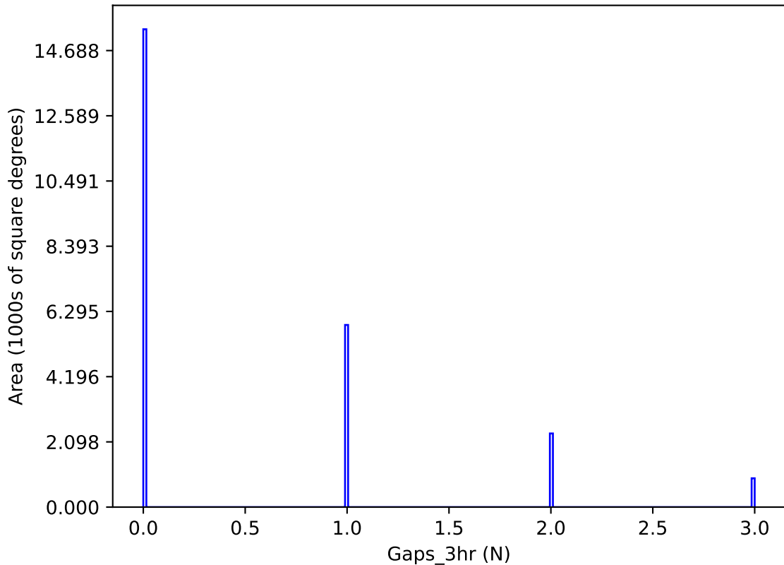
noroll_mjdp180_v3.4_10yrs y band: Gaps_3hr
