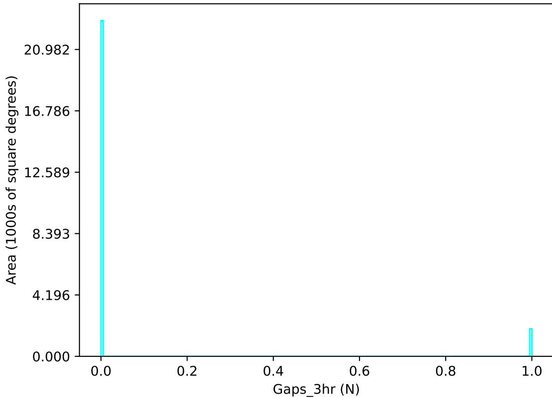
noroll_mjdp180_v3.4_10yrs u band: Gaps_3hr
