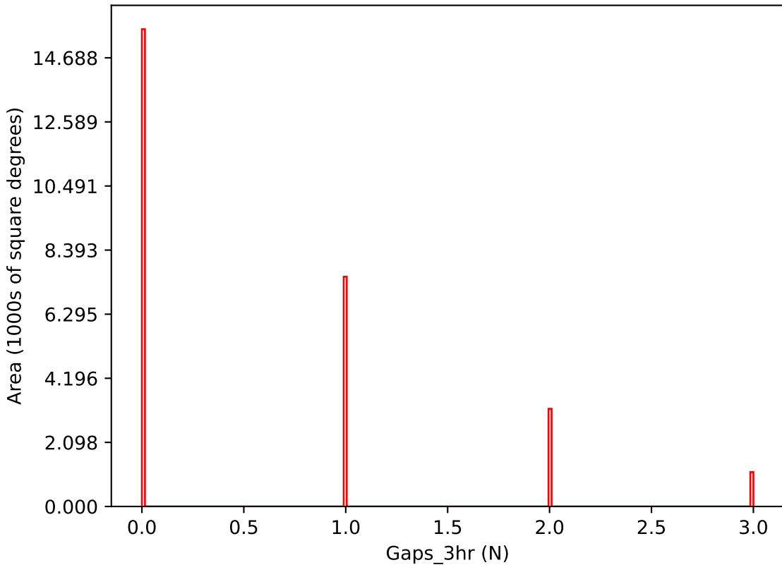
noroll_mjdp180_v3.4_10yrs i band: Gaps_3hr
