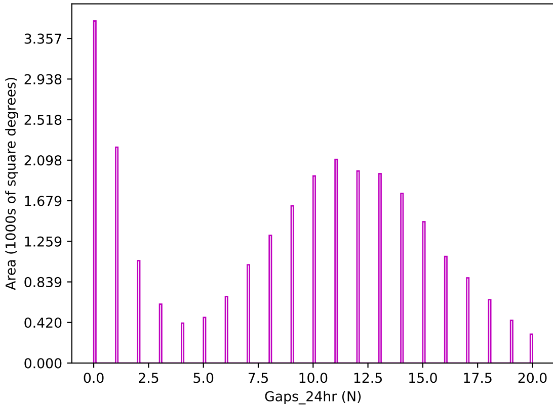
noroll_mjdp180_v3.4_10yrs z band: Gaps_24hr
