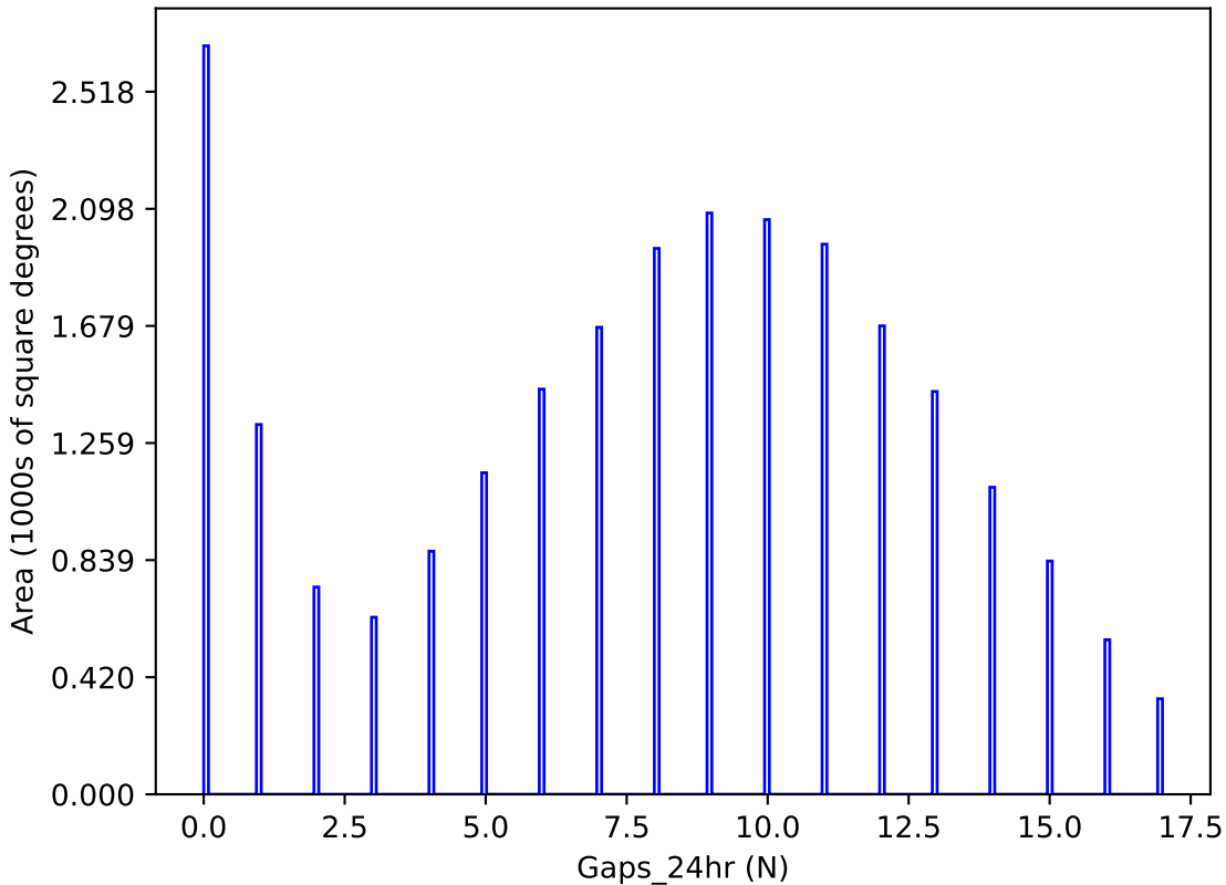
noroll_mjdp180_v3.4_10yrs y band: Gaps_24hr
