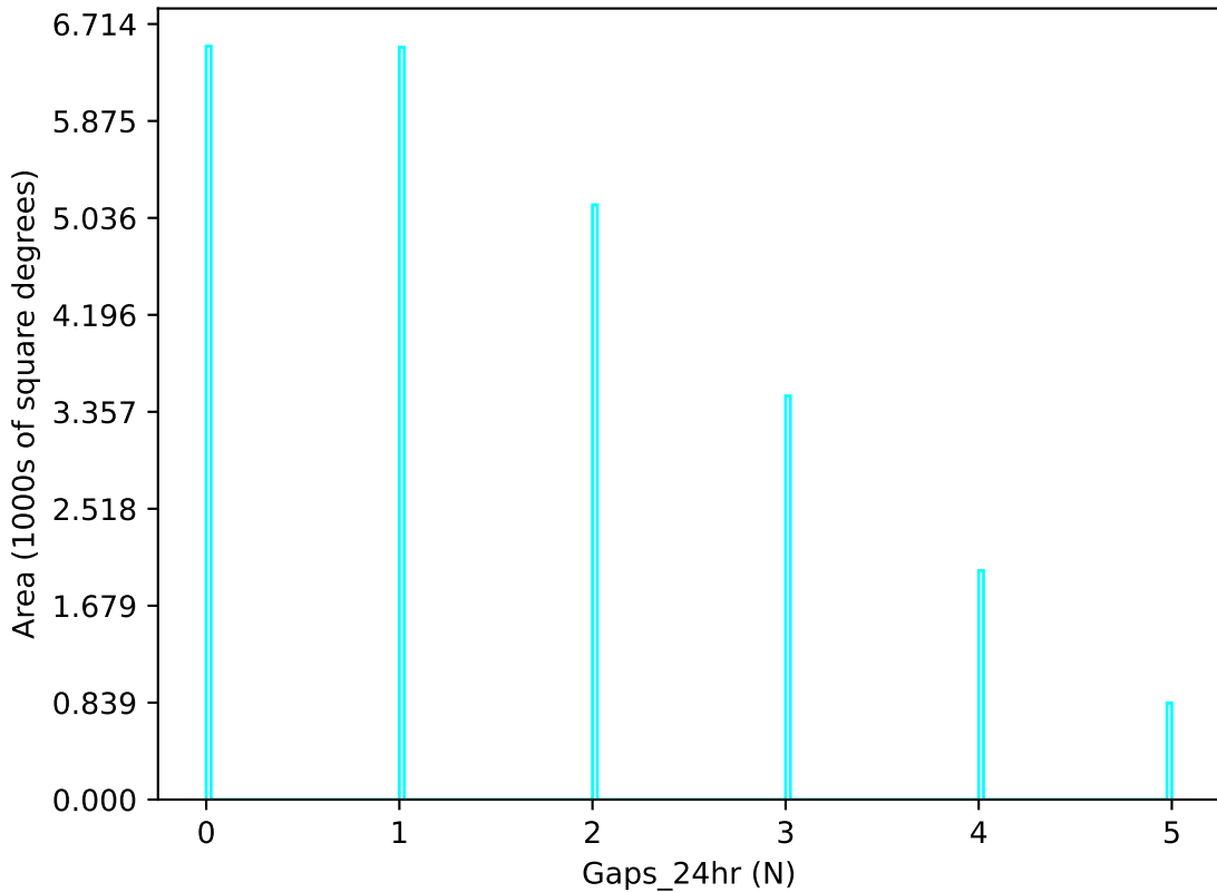
noroll_mjdp180_v3.4_10yrs u band: Gaps_24hr
