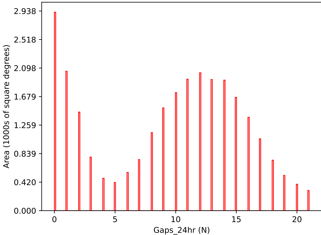
noroll_mjdp180_v3.4_10yrs i band: Gaps_24hr
