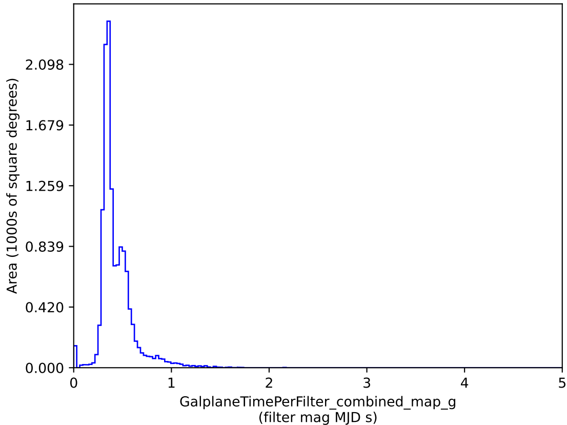
noroll_mjdp180_v3.4_10yrs : GalplaneTimePerFilter_combined_map_g
