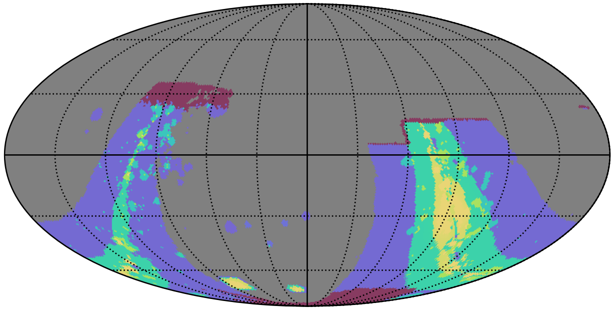
noroll_mjdp180_v3.4_10yrs : GalplaneFootprintMetric_combined_map_Tau_46_5
