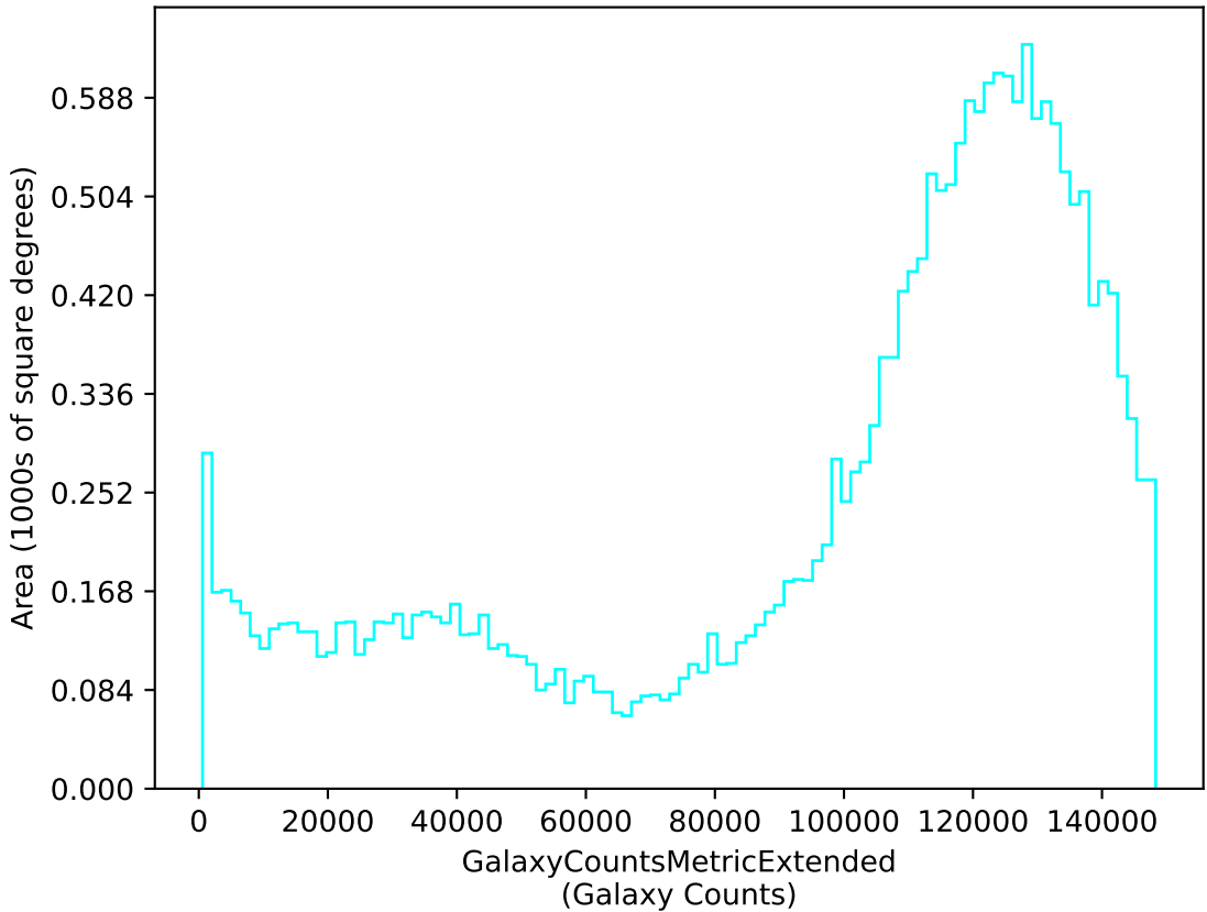
noroll_mjdp180_v3.4_10yrs u: GalaxyCountsMetricExtended
