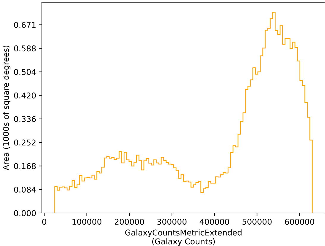
noroll_mjdp180_v3.4_10yrs r: GalaxyCountsMetricExtended
