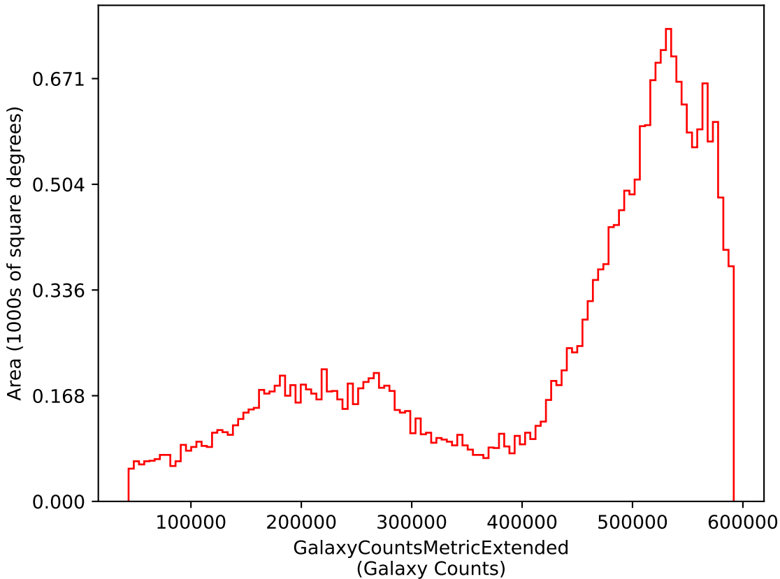
noroll_mjdp180_v3.4_10yrs i: GalaxyCountsMetricExtended
