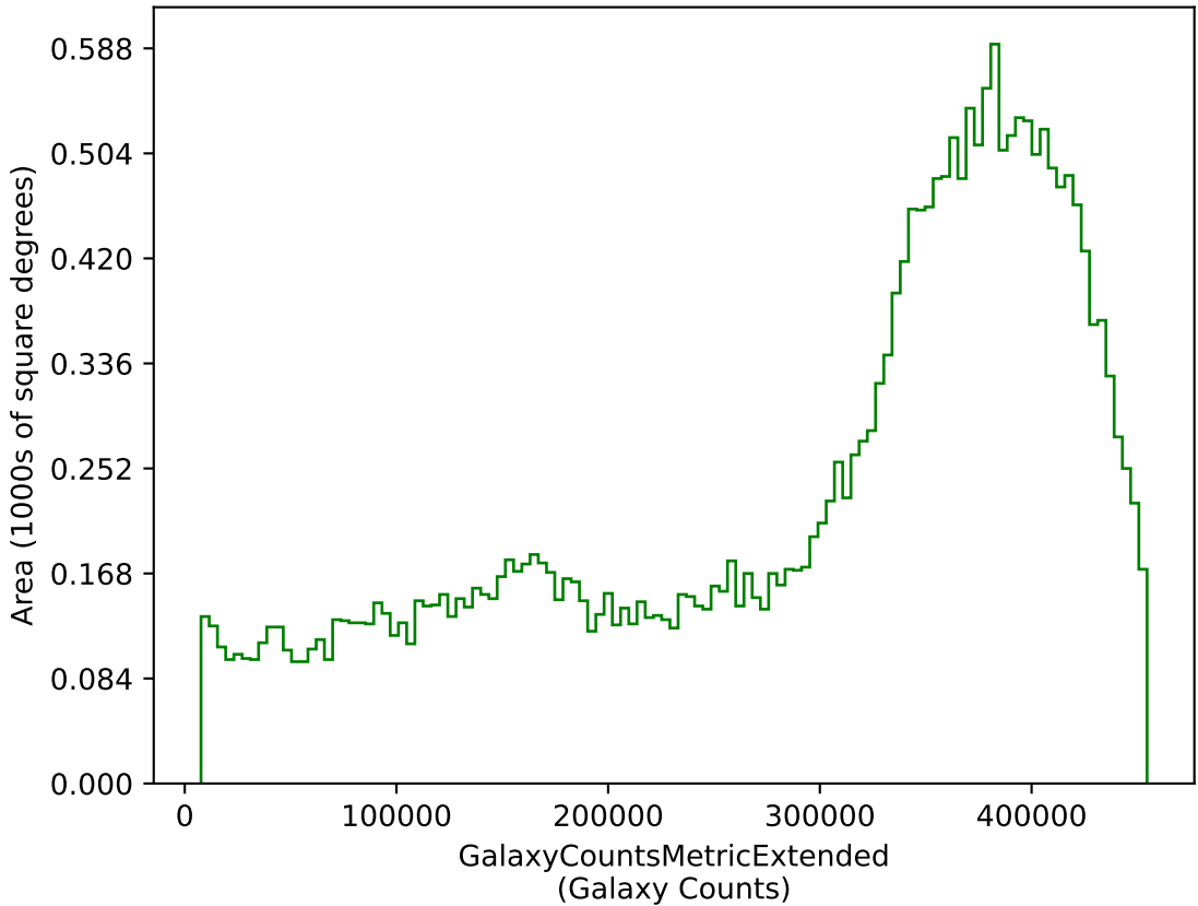
noroll_mjdp180_v3.4_10yrs g: GalaxyCountsMetricExtended
