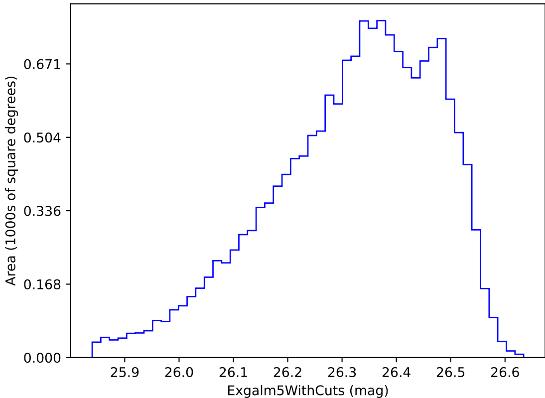
noroll_mjdp180_v3.4_10yrs i band non-DD year 9: ExgalM5WithCuts
