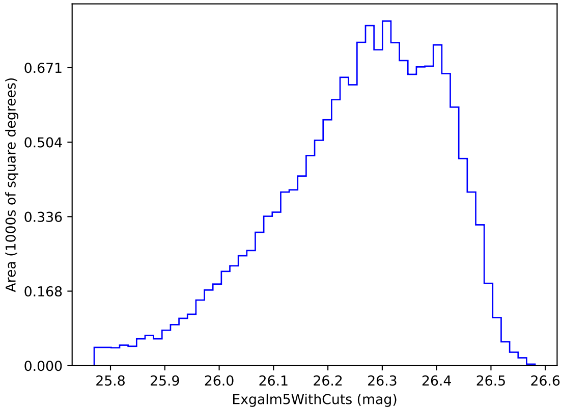
noroll_mjdp180_v3.4_10yrs i band non-DD year 8: ExgalM5WithCuts
