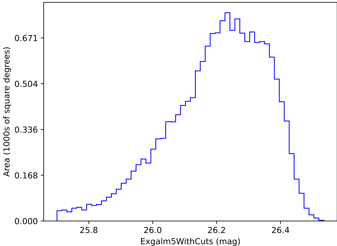
noroll_mjdp180_v3.4_10yrs i band non-DD year 7: ExgalM5WithCuts
