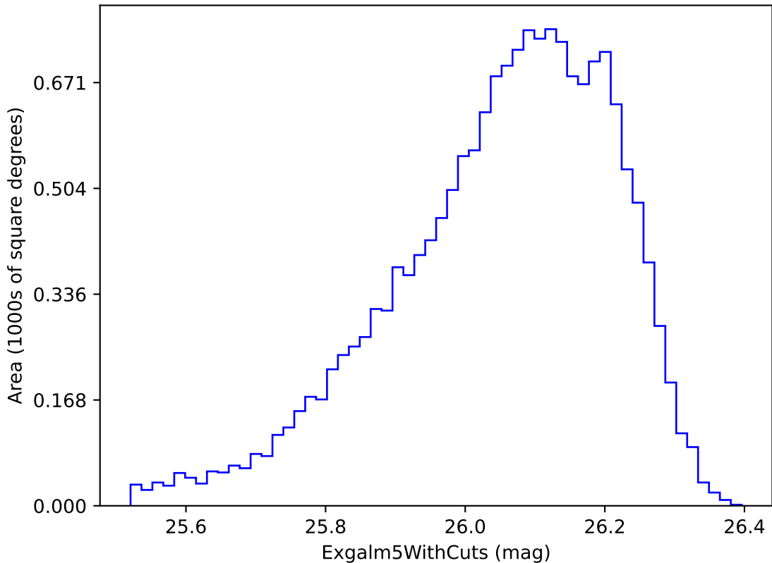
noroll_mjdp180_v3.4_10yrs i band non-DD year 5: ExgalM5WithCuts
