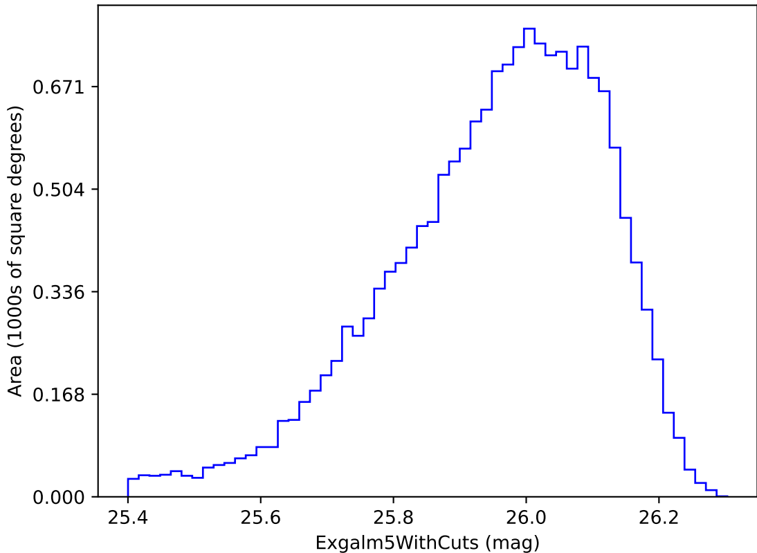
noroll_mjdp180_v3.4_10yrs i band non-DD year 4: ExgalM5WithCuts
