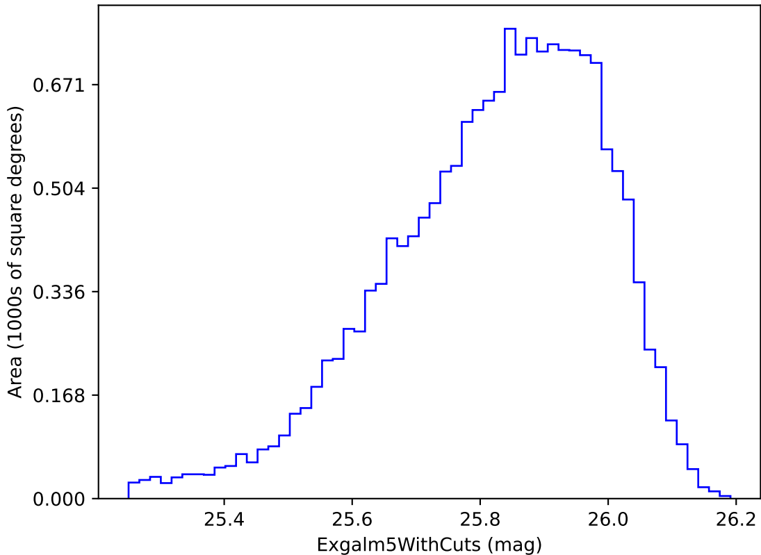
noroll_mjdp180_v3.4_10yrs i band non-DD year 3: ExgalM5WithCuts
