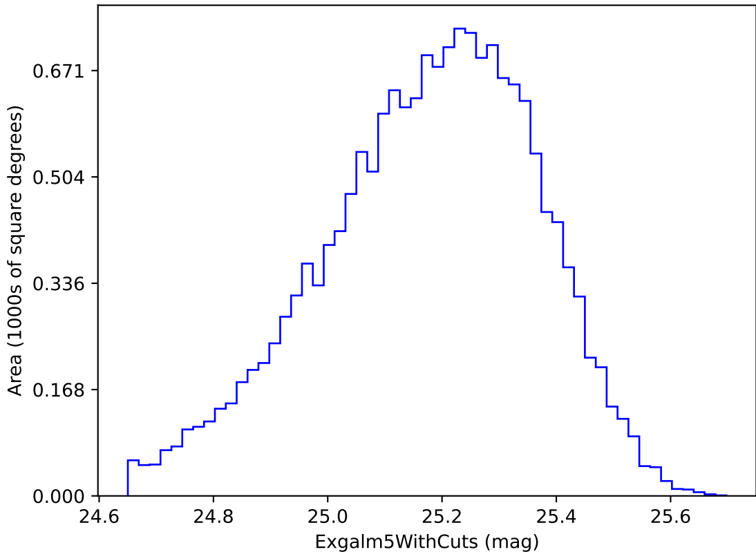
noroll_mjdp180_v3.4_10yrs i band non-DD year 1: ExgalM5WithCuts
