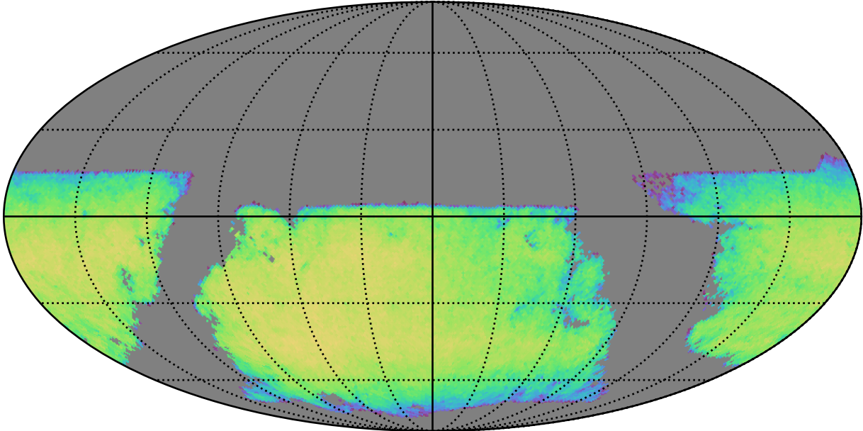
noroll_mjdp180_v3.4_10yrs i band galaxies non-DD: DepthLimitedNumGalaxiesMetric
