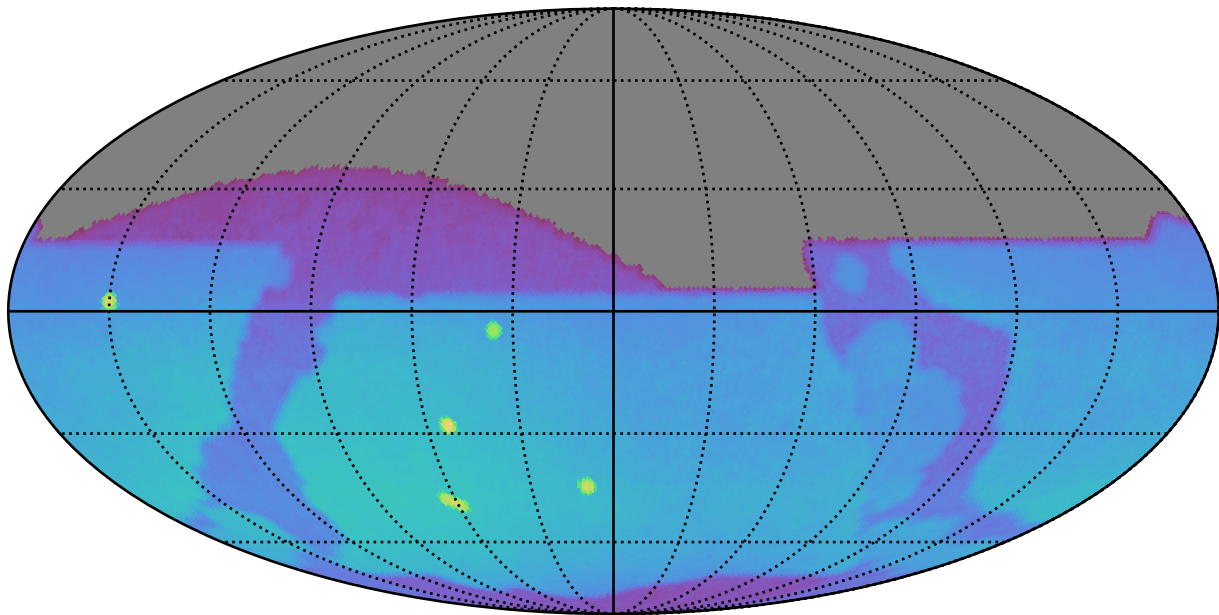
noroll_mjdp180_v3.4_10yrs : Brown Dwarf, L7
