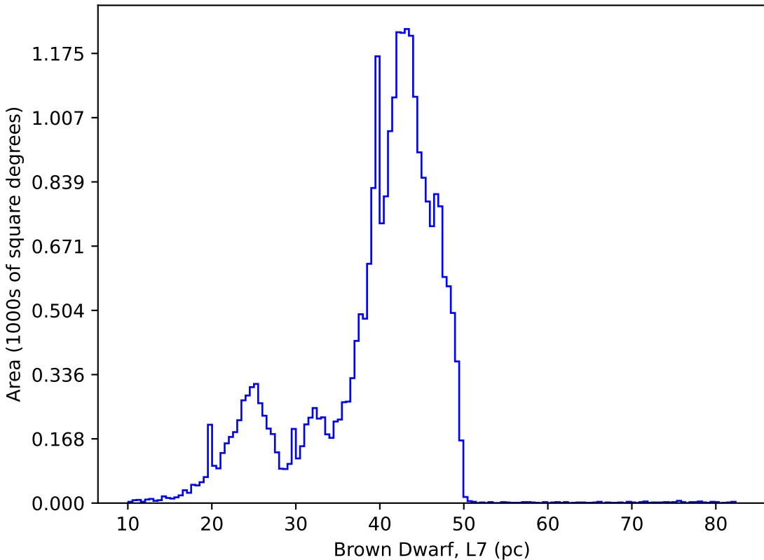
noroll_mjdp180_v3.4_10yrs : Brown Dwarf, L7
