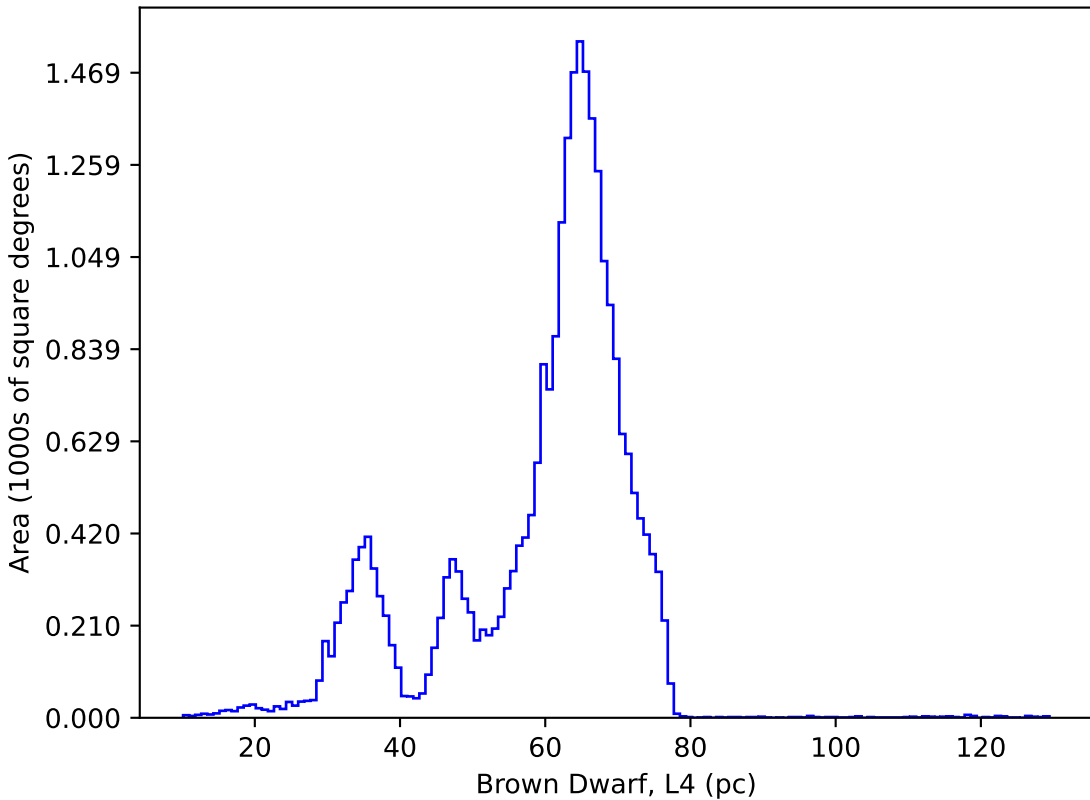
noroll_mjdp180_v3.4_10yrs : Brown Dwarf, L4
