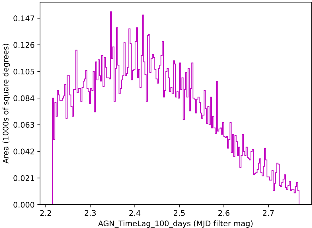
noroll_mjdp180_v3.4_10yrs z band: AGN_TimeLag_100_days
