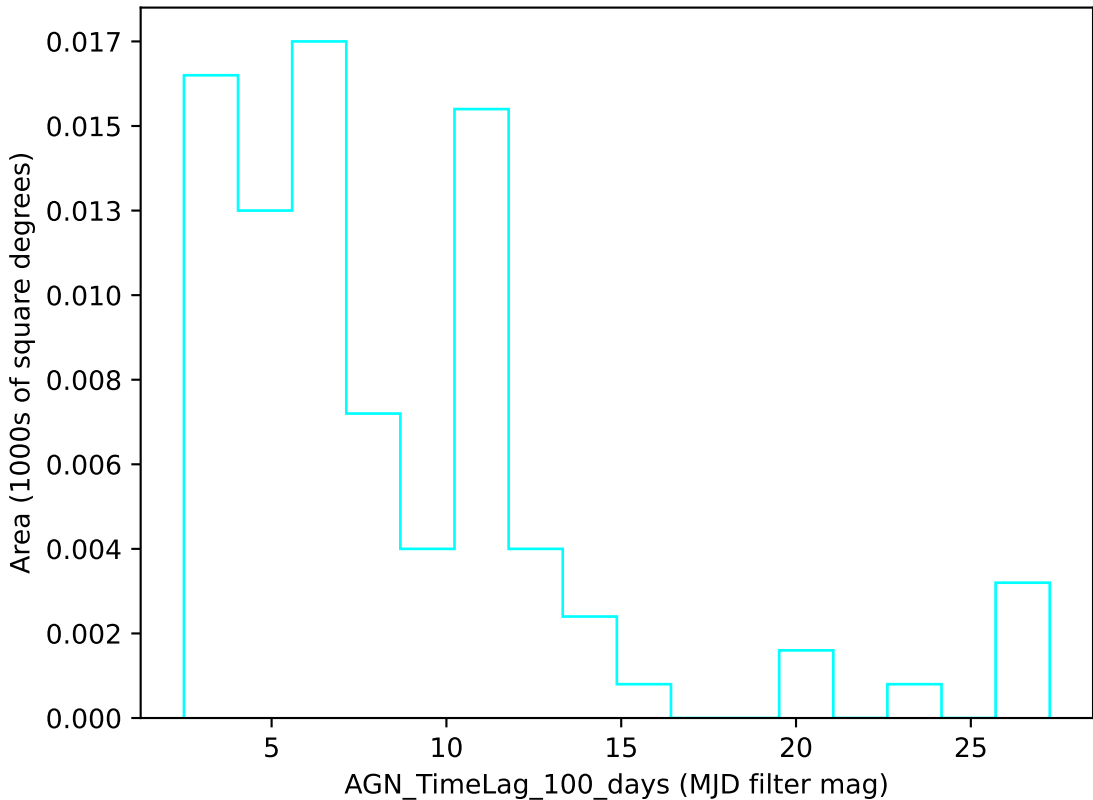
noroll_mjdp180_v3.4_10yrs u band: AGN_TimeLag_100_days
