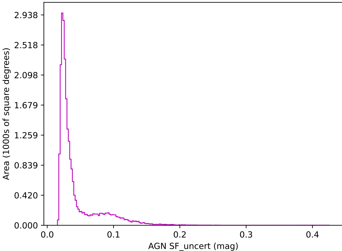
noroll_mjdp180_v3.4_10yrs z band: AGN SF_uncert
