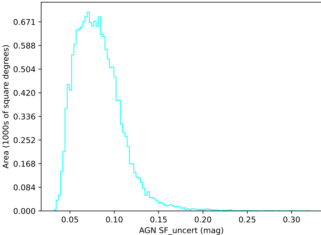
noroll_mjdp180_v3.4_10yrs u band: AGN SF_uncert
