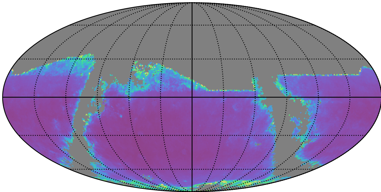
noroll_mjdp180_v3.4_10yrs r band: AGN SF_uncert
