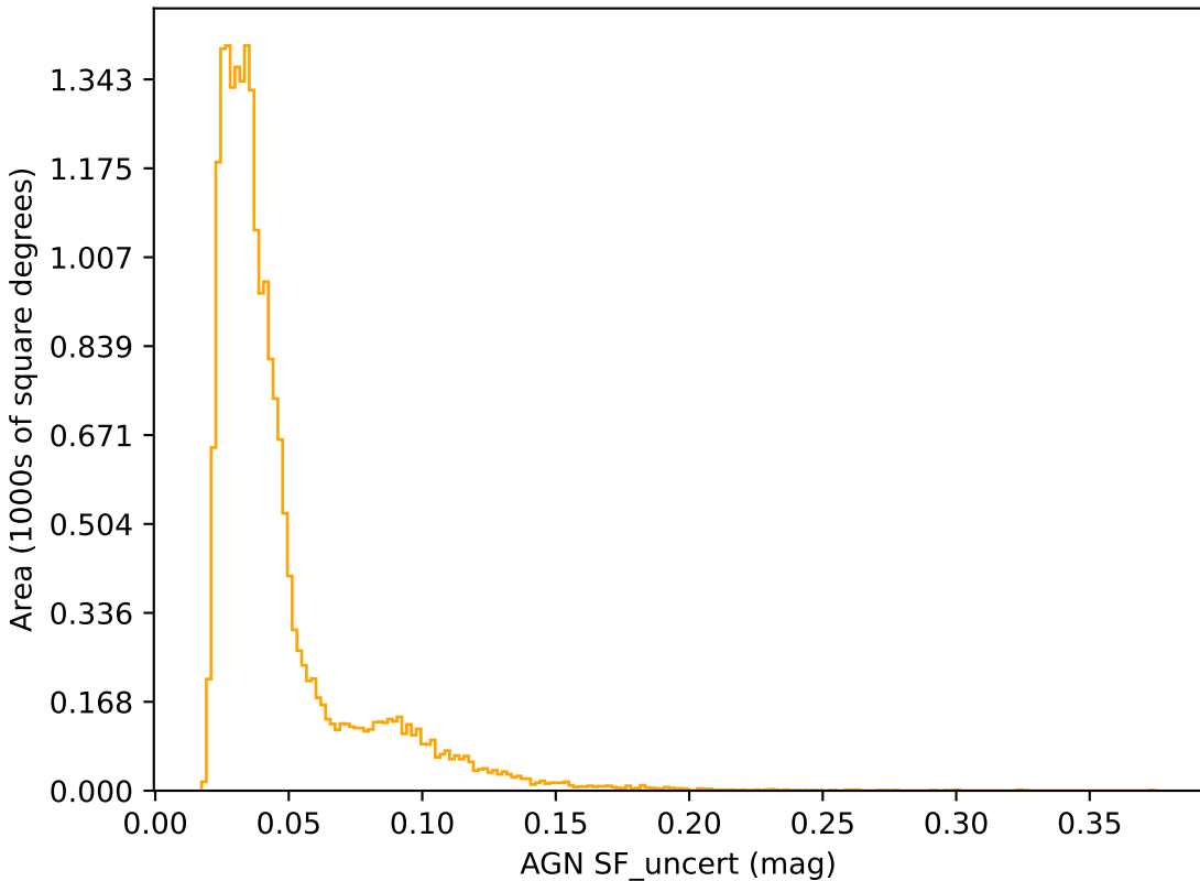
noroll_mjdp180_v3.4_10yrs r band: AGN SF_uncert
