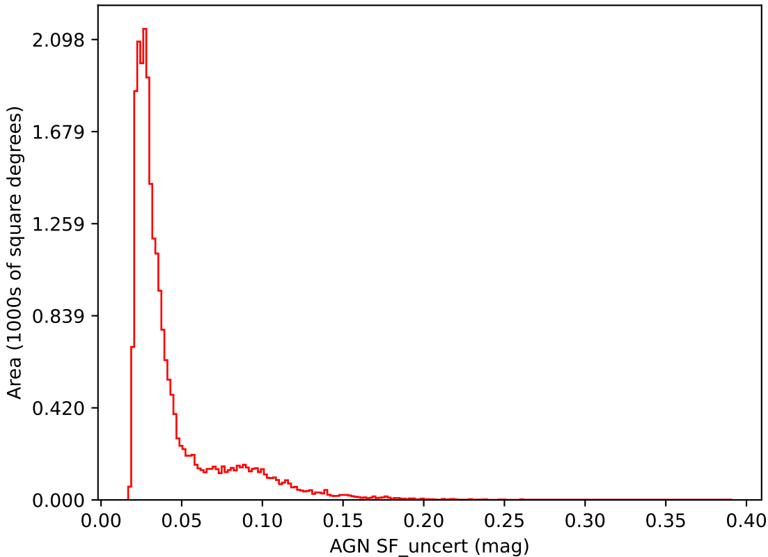
noroll_mjdp180_v3.4_10yrs i band: AGN SF_uncert
