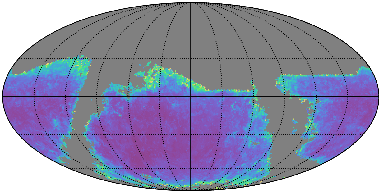
noroll_mjdp180_v3.4_10yrs g band: AGN SF_uncert
