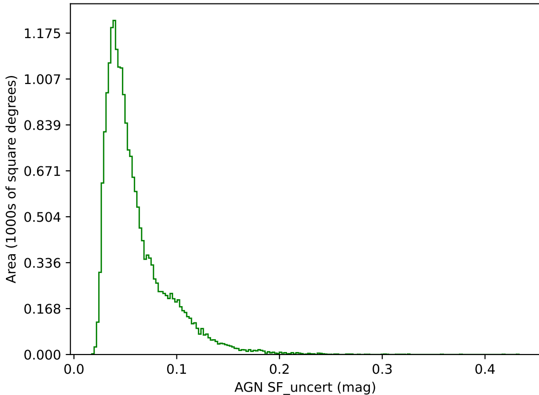
noroll_mjdp180_v3.4_10yrs g band: AGN SF_uncert
