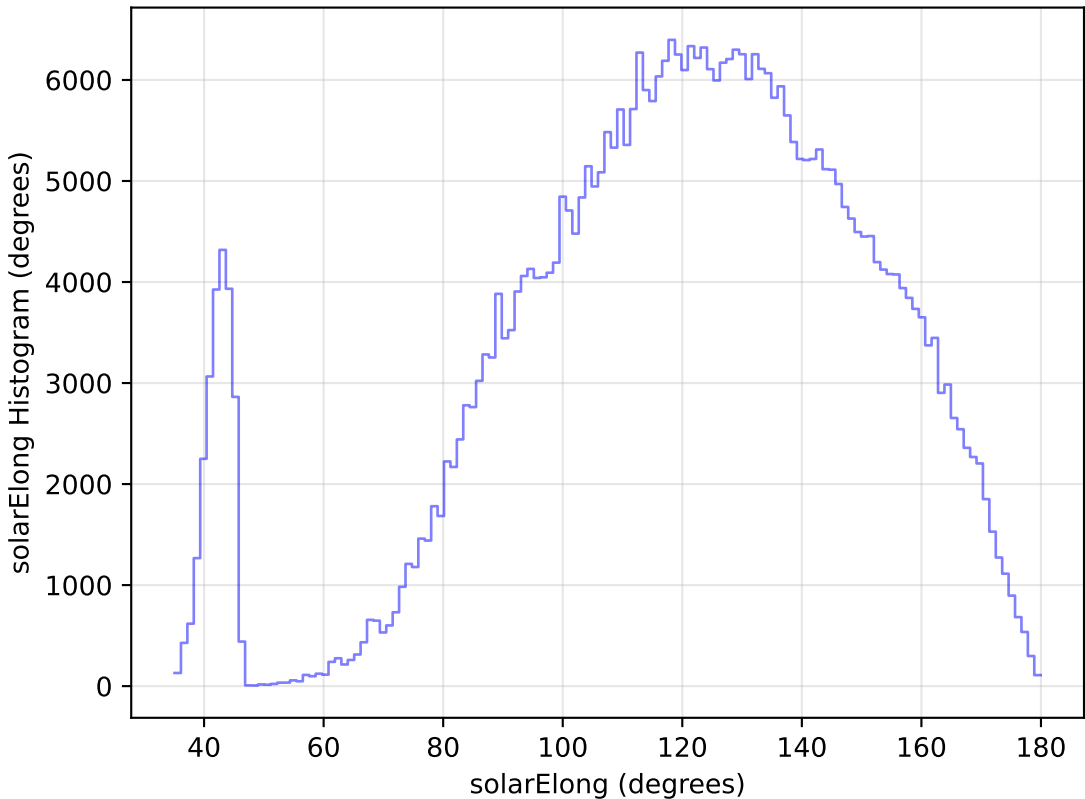
noroll_mjdp180_v3.4_10yrs WFD z band: solarElong Histogram
