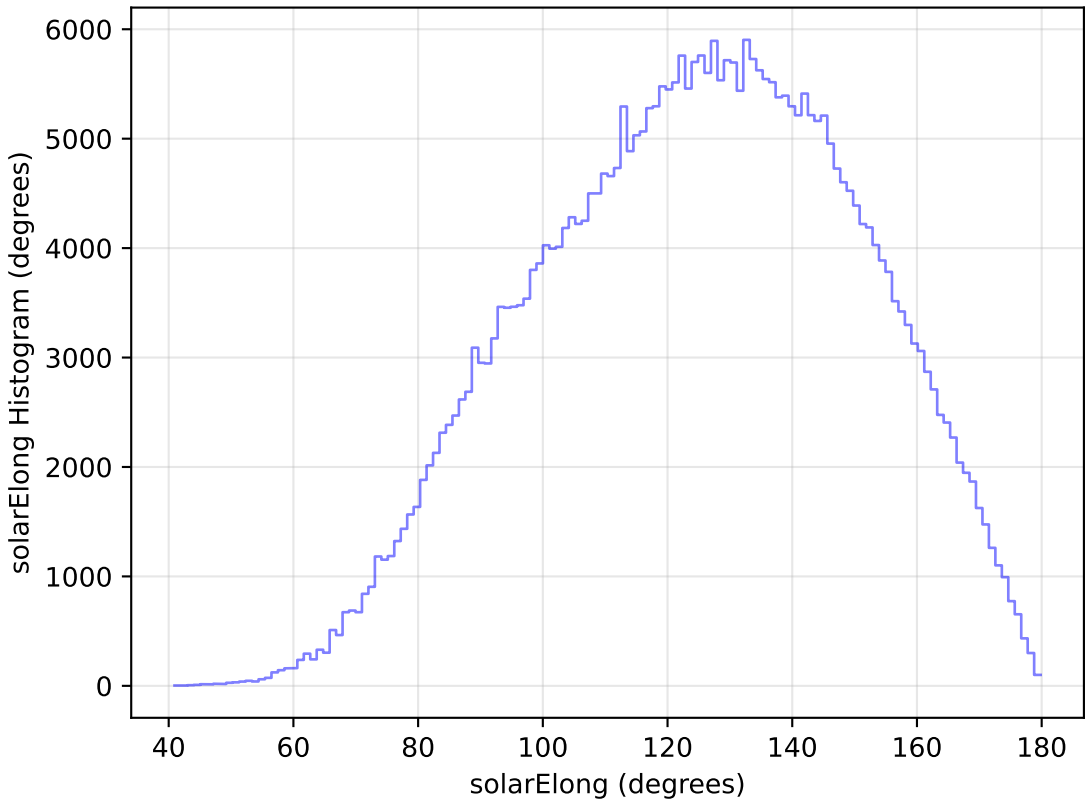
noroll_mjdp180_v3.4_10yrs WFD y band: solarElong Histogram
