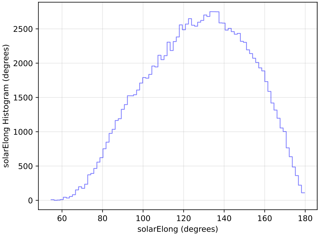
noroll_mjdp180_v3.4_10yrs WFD u band: solarElong Histogram
