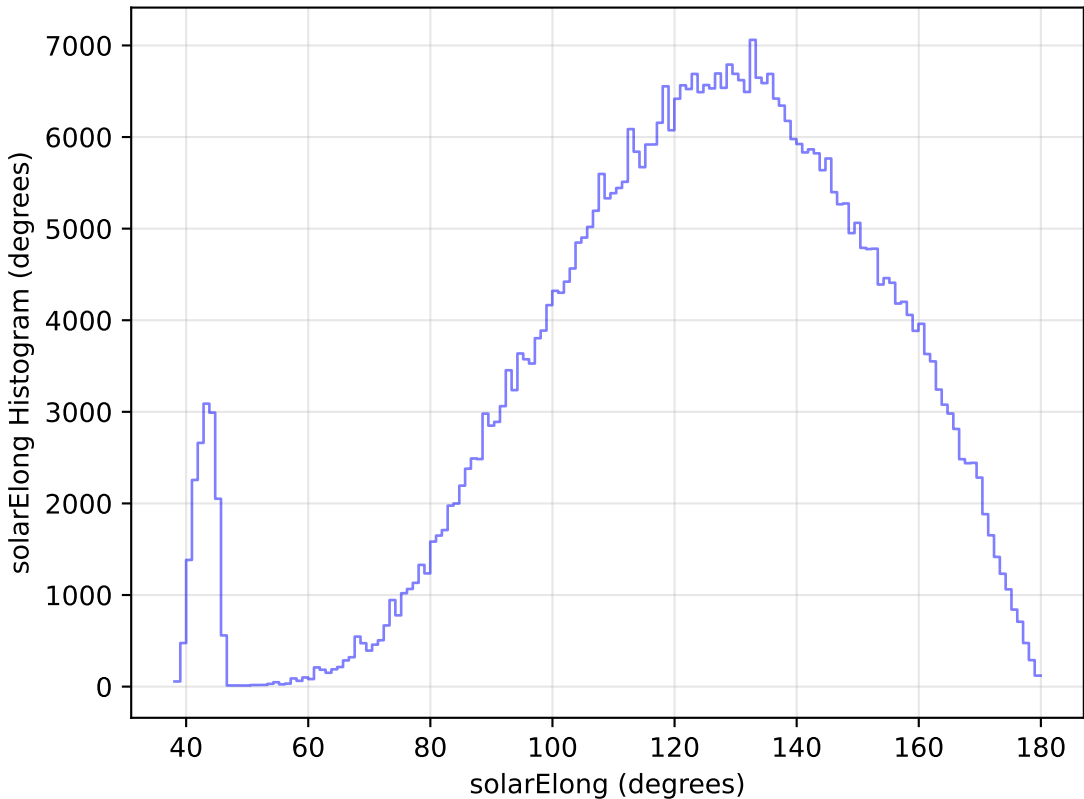
noroll_mjdp180_v3.4_10yrs WFD r band: solarElong Histogram
