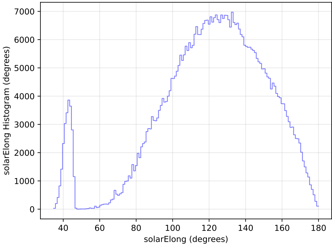
noroll_mjdp180_v3.4_10yrs WFD i band: solarElong Histogram
