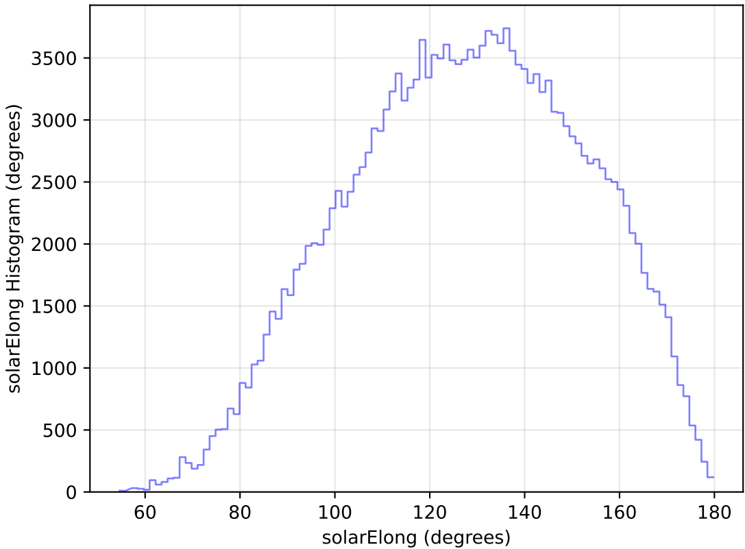
noroll_mjdp180_v3.4_10yrs WFD g band: solarElong Histogram
