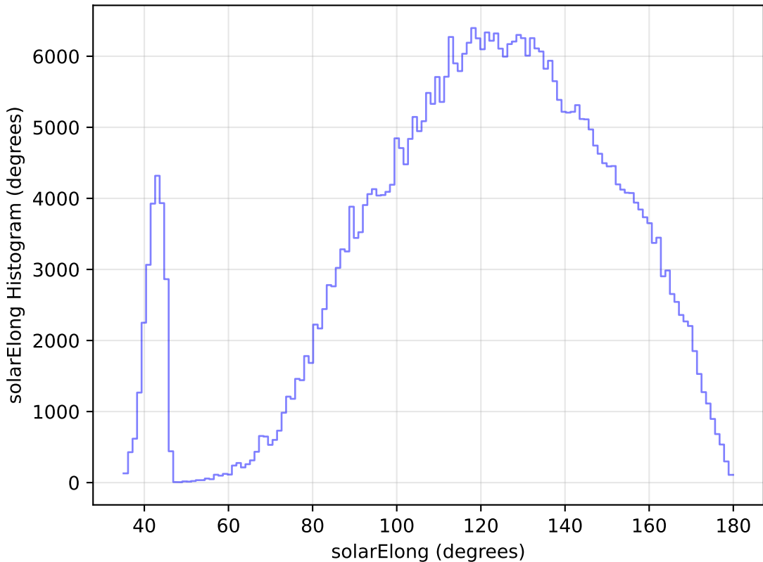
noroll_mjdp180_v3.4_10yrs All sky z band: solarElong Histogram
