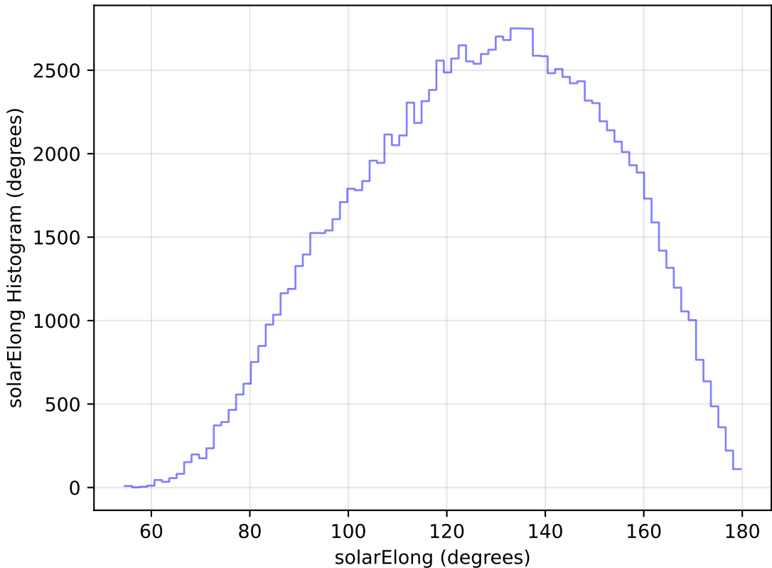
noroll_mjdp180_v3.4_10yrs All sky u band: solarElong Histogram
