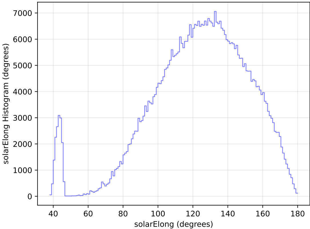
noroll_mjdp180_v3.4_10yrs All sky r band: solarElong Histogram
