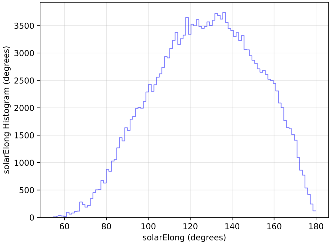
noroll_mjdp180_v3.4_10yrs All sky g band: solarElong Histogram
