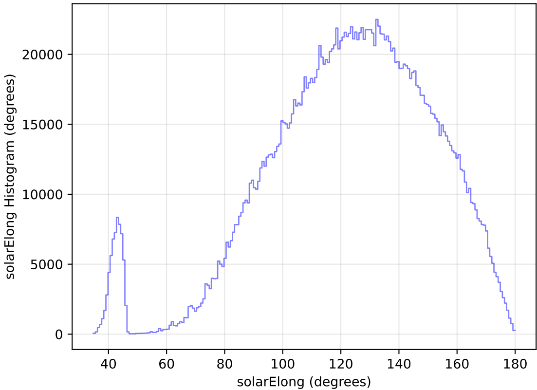
noroll_mjdp180_v3.4_10yrs All sky all bands: solarElong Histogram
