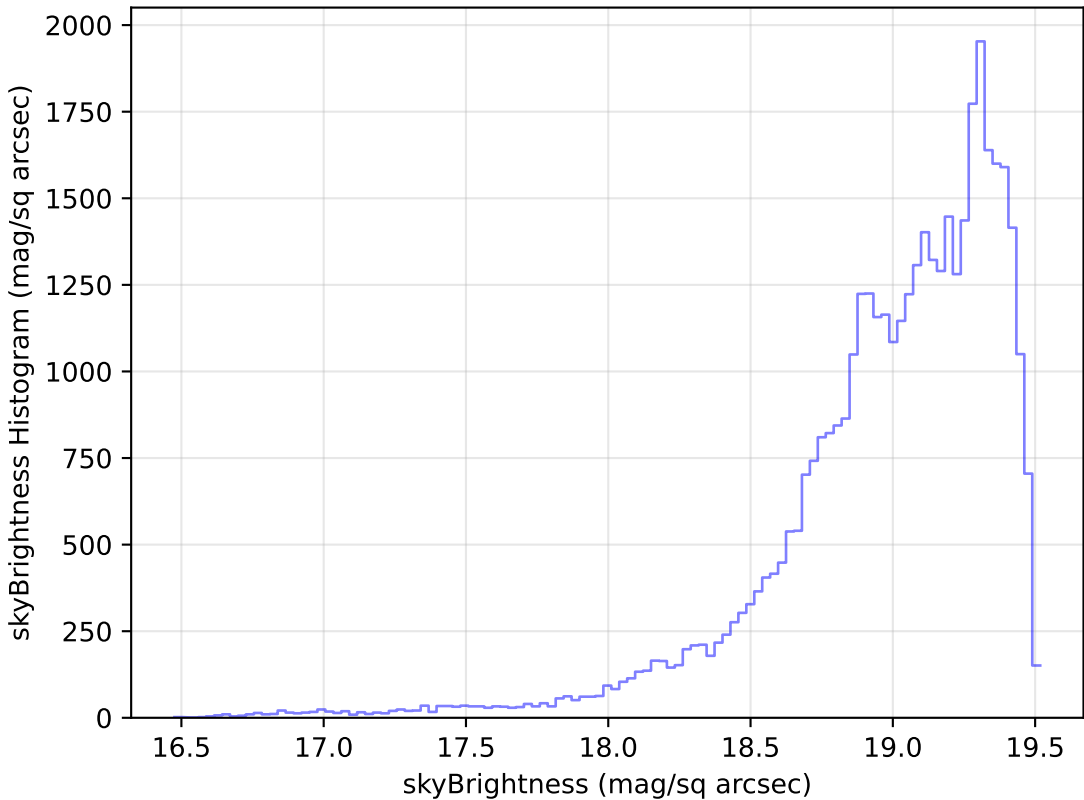
noroll_mjdp180_v3.4_10yrs Yr 1 z band: skyBrightness Histogram
