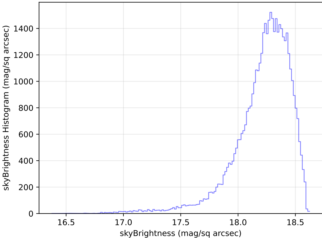
noroll_mjdp180_v3.4_10yrs Yr 1 y band: skyBrightness Histogram
