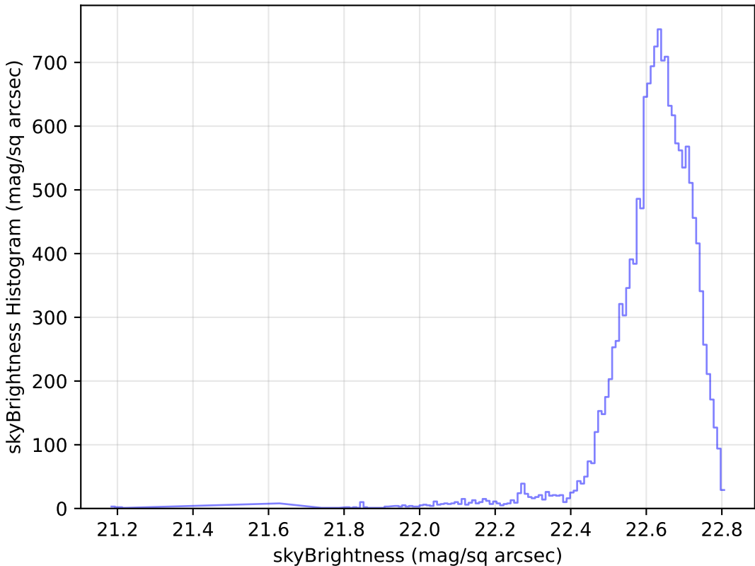
noroll_mjdp180_v3.4_10yrs Yr 1 u band: skyBrightness Histogram
